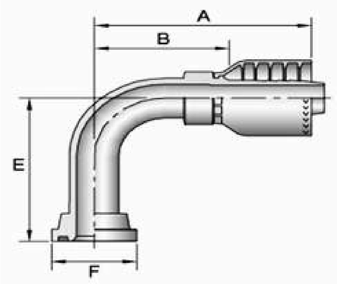
189GM SAE Code 61 Flange Head 90° Long Drop Elbow
